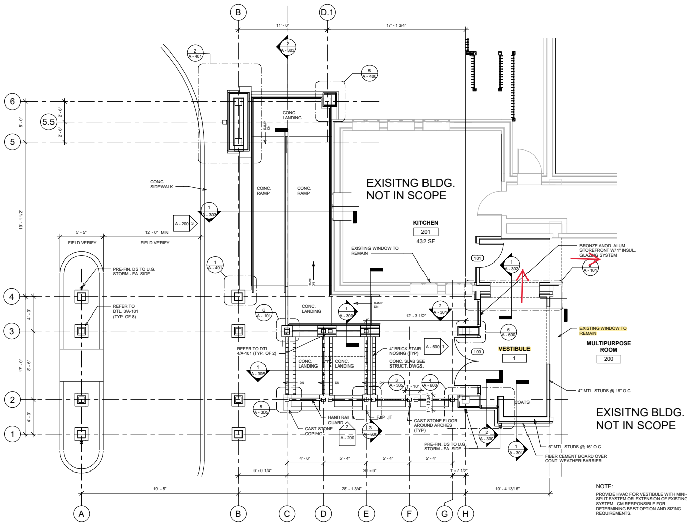
1 ENTRY LEVEL FLOOR PLAN 1/4" = 1'-0"
